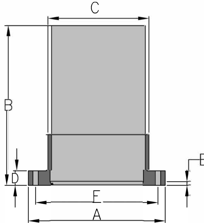
ELEVATION VIEW
