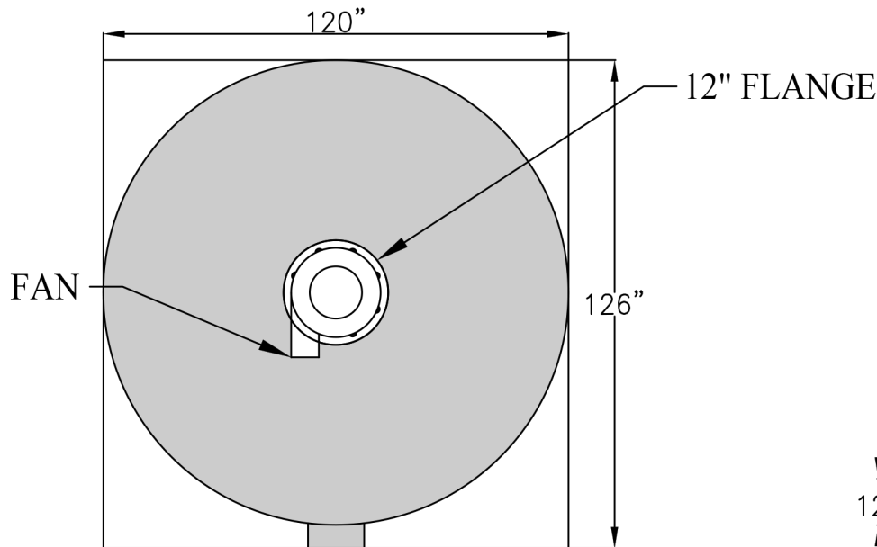
TOP VIEW
