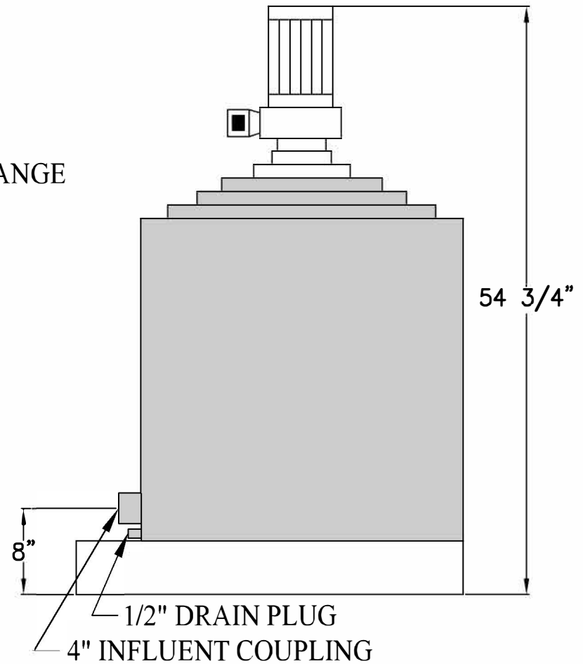
SIDE VIEW
