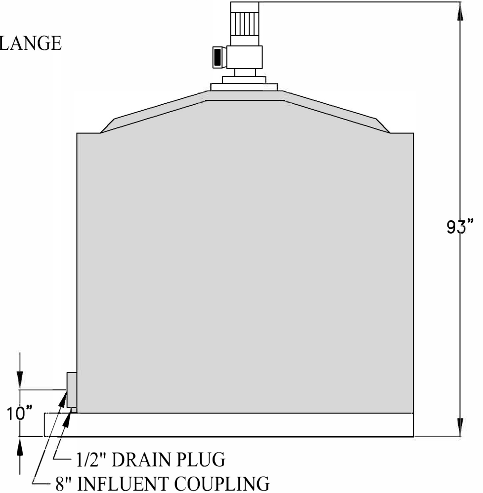
SIDE VIEW
