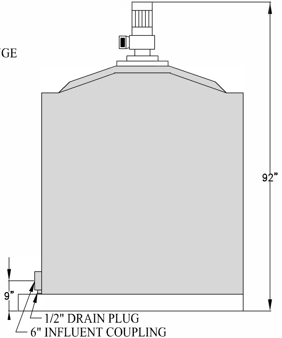
SIDE VIEW
