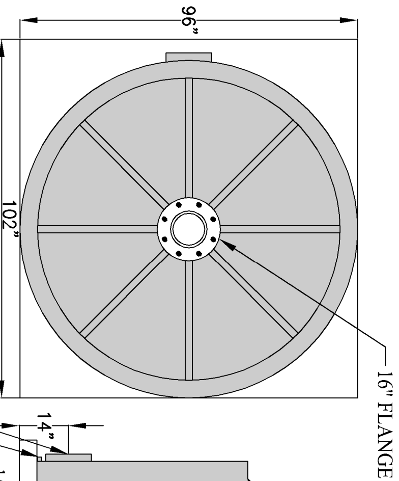
TOP VIEW
